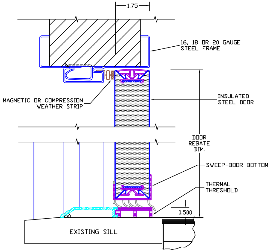
SILL DETAIL
